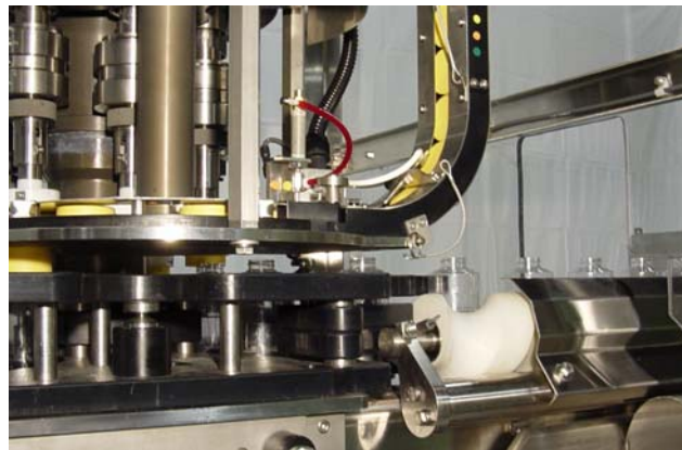
Infeed Screw/Cap Chute
